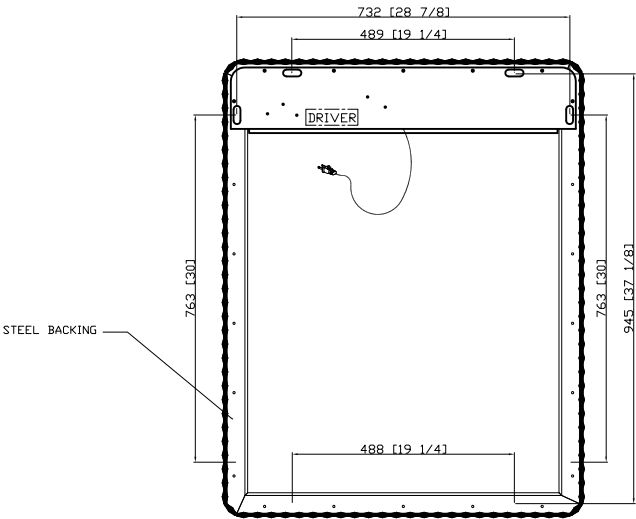
SECTION - FRONT
