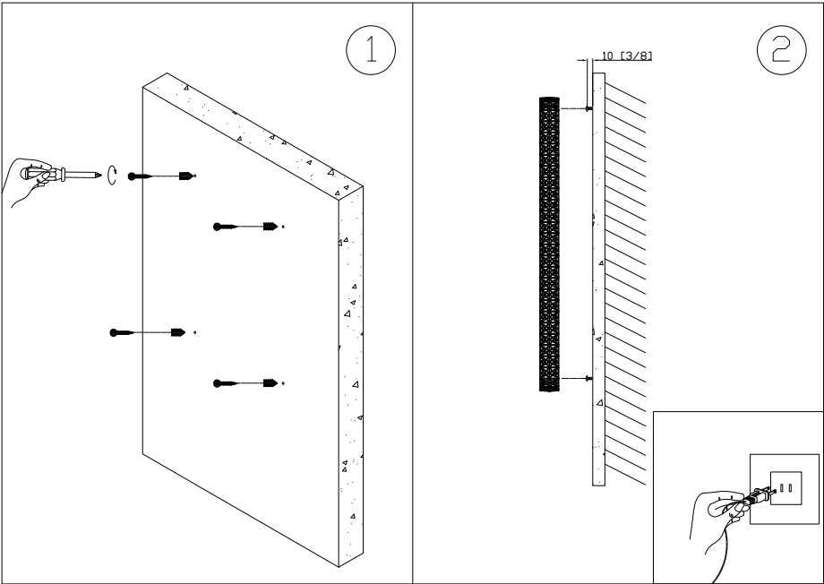
WALL INSTALLATION DIAGRAM
