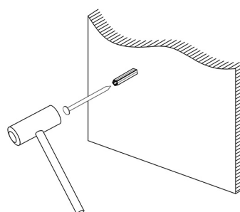
Step 4: Nail the screw into the expanded rubber cap, with the nail head reserved for 5mm, and hang the product back hook or hanging chain on the screw to finish.
