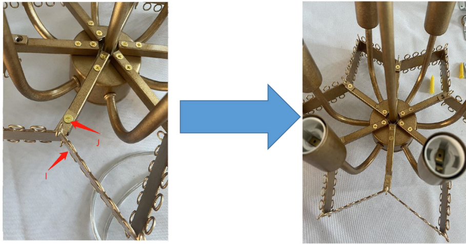
Step 5: Fix I with the screw J
