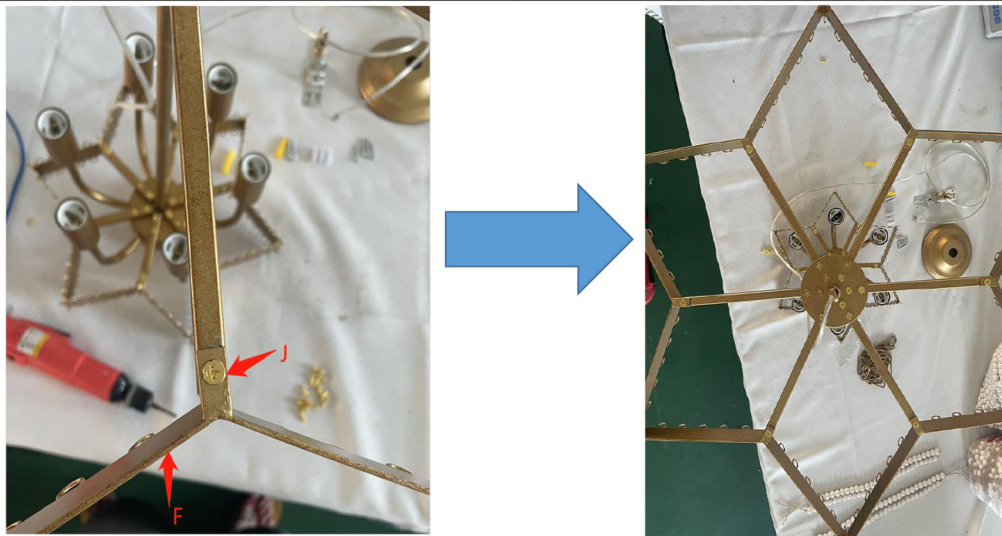
Step 6: Fix F with the screw J
