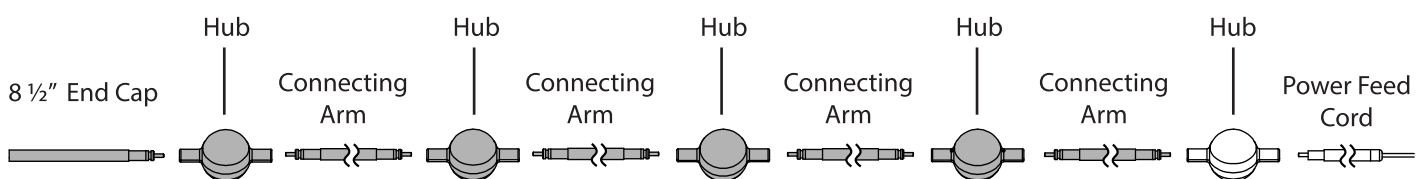
Fig. 2d - Long Drop
